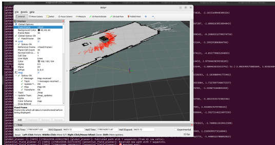
Fig. 3: Particle filter visualization: Red arrows represent particle hypotheses clustering around the robot
